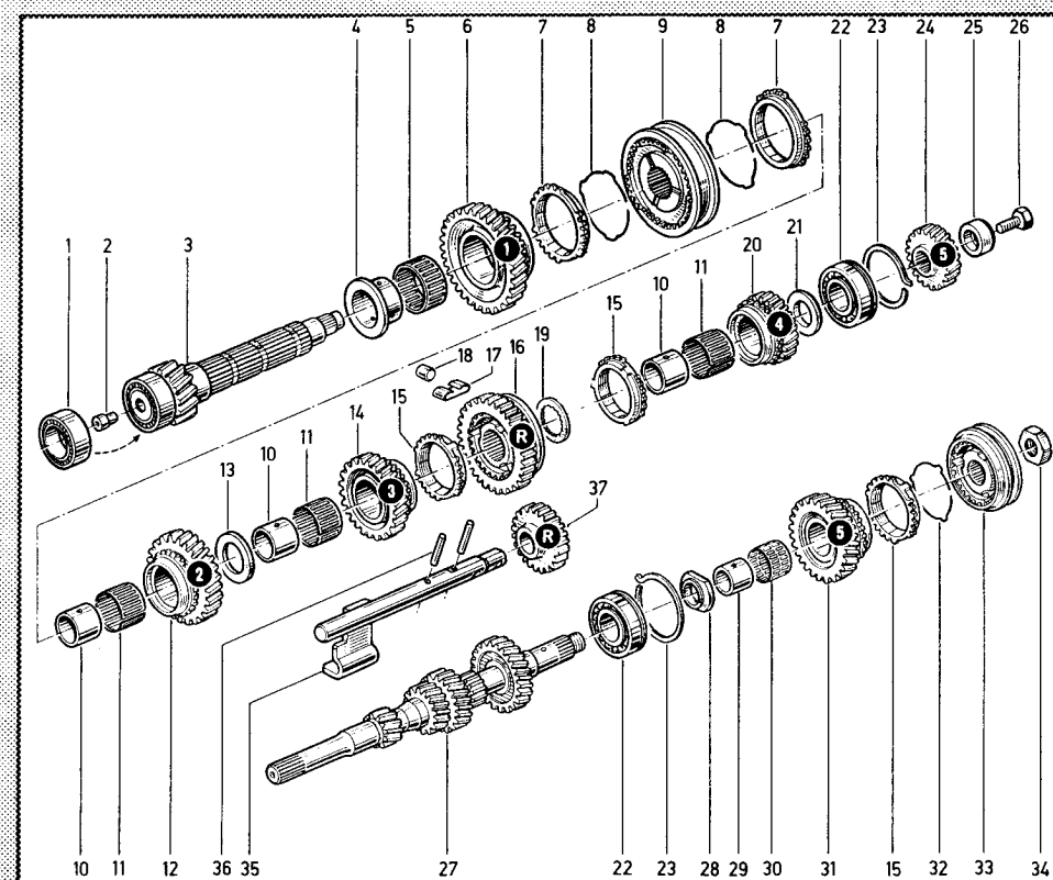
Ensemble pignonnerie
