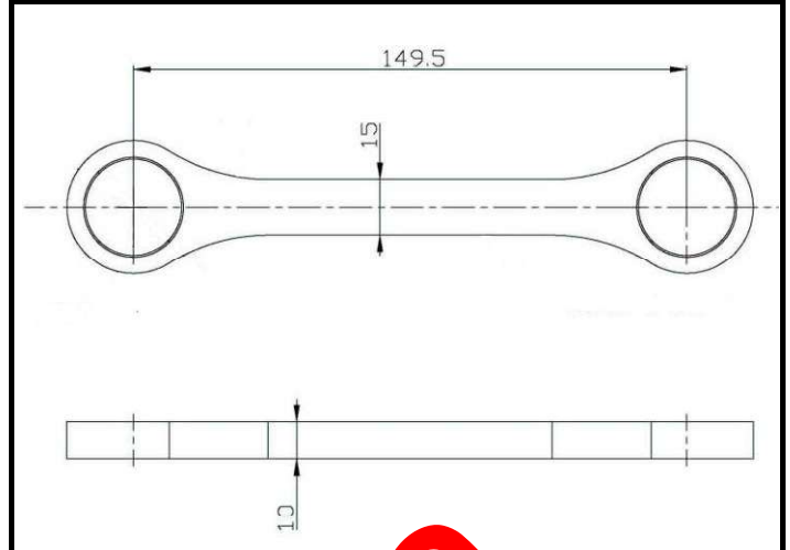
SM3) Support N°3 (Drawing)
